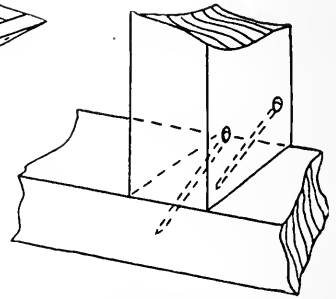
TOE NAIL JOINT
